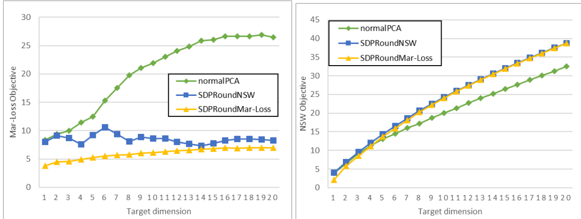
Figure 4.4: Marginal loss and NSW objective of standard PCA compared to our SDP-based algorithms on Adult Income data. SDPRoundNSW and SDPRoundMar-Loss are two runs of the SDP algorithms maximizing NSW objective and minimizing maximum marginal loss.
