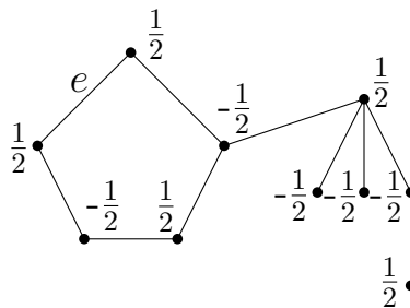
Figure 2.1: The values of the coordinates of u_e for e \in C_\ell .
