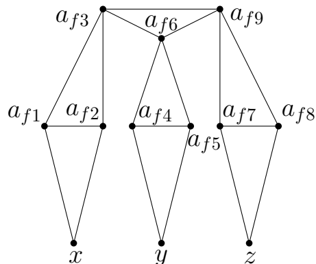
Figure 2.3: The subgraph with edges E_f for the triple f = \{x, y, z\} . (Adapted from [GJ79])
