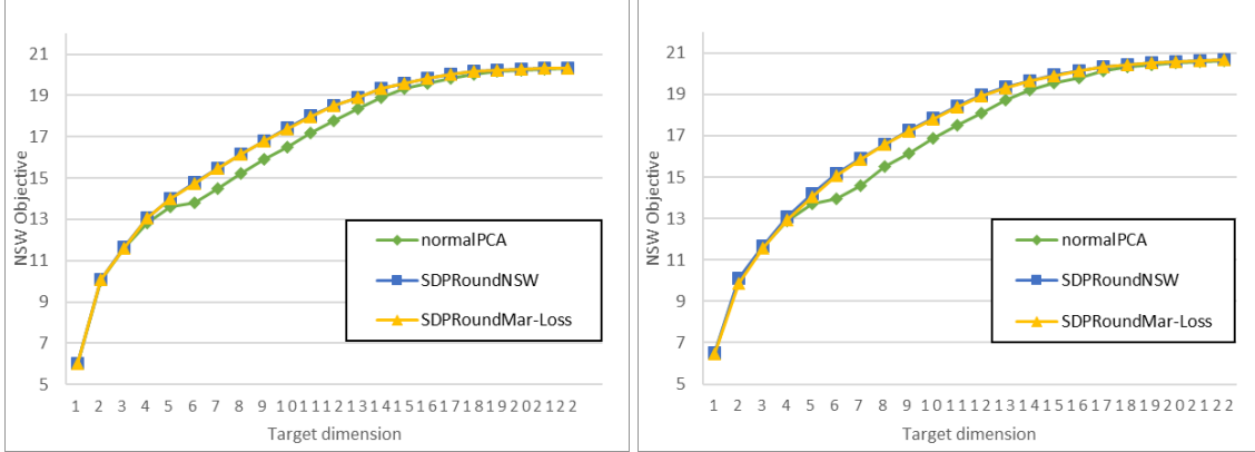
Figure 4.3: NSW objective of standard PCA compared to our SDP-based algorithms on Default Credit data. SDPRoundNSW and SDPRoundMar-Loss are two runs of the SDP algorithms maximizing NSW objective and minimizing maximum marginal loss. Left: k = 4 groups. Right: k = 6 .
