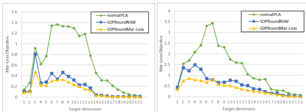
Figure 4.2: Marginal loss function of standard PCA compared to our SDP-based algorithms on Default Credit data. SDPRoundNSW and SDPRoundMar-Loss are two runs of the SDP-based algorithms maximizing NSW and minimizing marginal loss. Left: k = 4 groups. Right: k = 6 .
